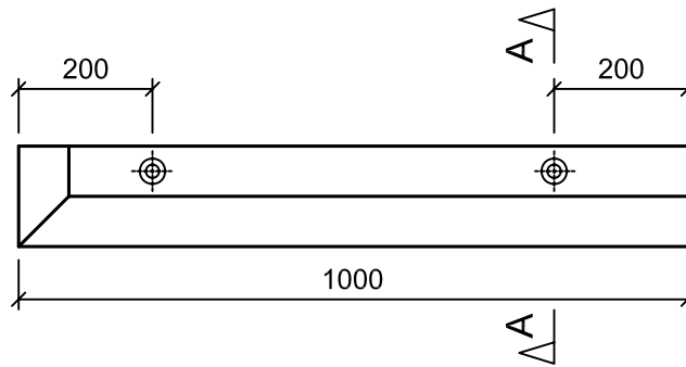
PLAN OF LEADING KERB AS DRAWN (TRAILING KERB IS OPP. HAND)
